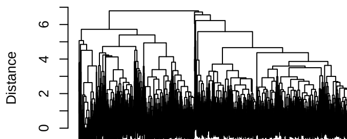
Manhattan + Average
