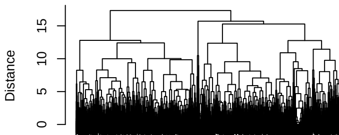
Manhattan + Complete
