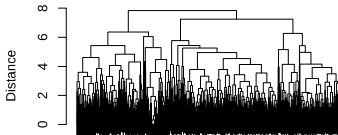
Euclidean + Complete
